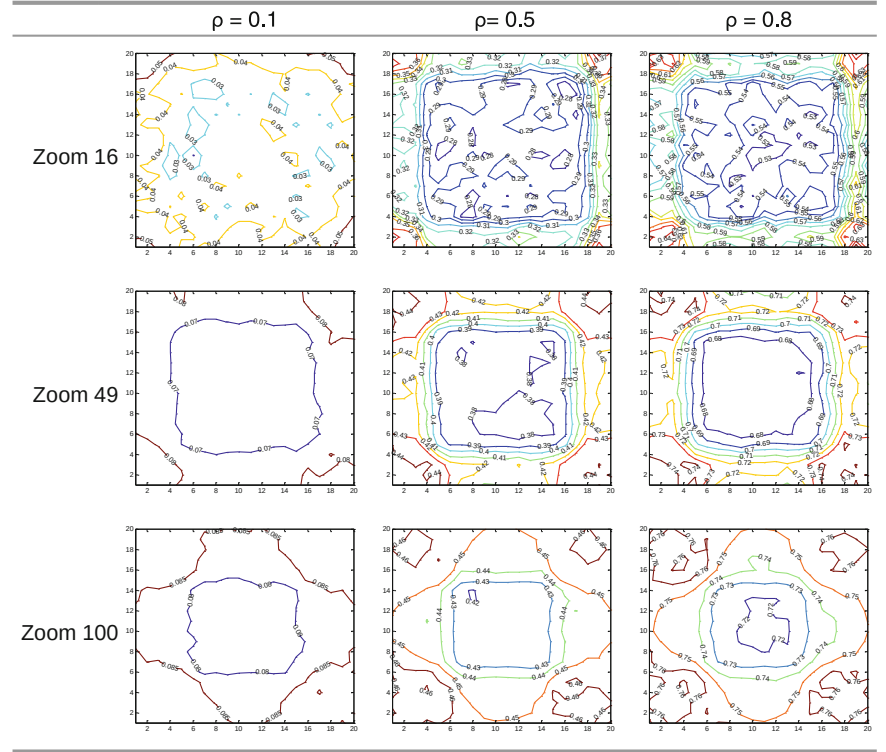
Fig. 3 Spatial distribution of \rho_r . Lattice 20 \times 20
