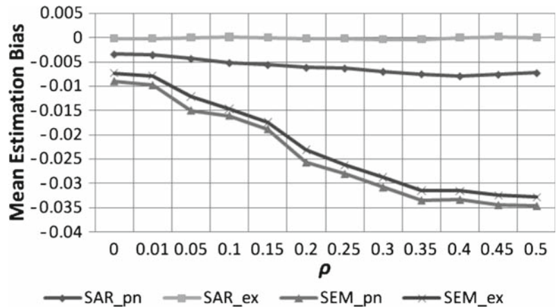
Fig. 8 Dependence parameter estimation bias for different levels of dependence
